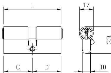
European double profile cylinder
