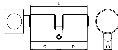
European double profile cylinder. Round knob
